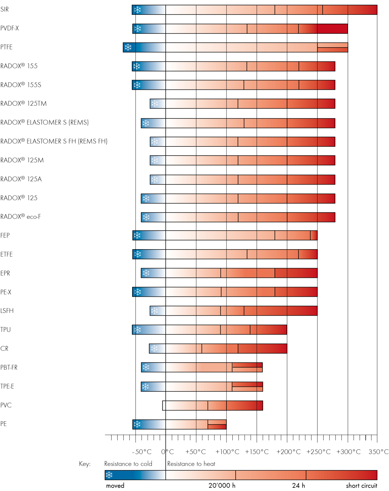
Typical operating temperature ranges of different insulations and sheaths
